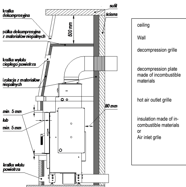
Picture 8. Exemplary installation of the fireplace insert.
