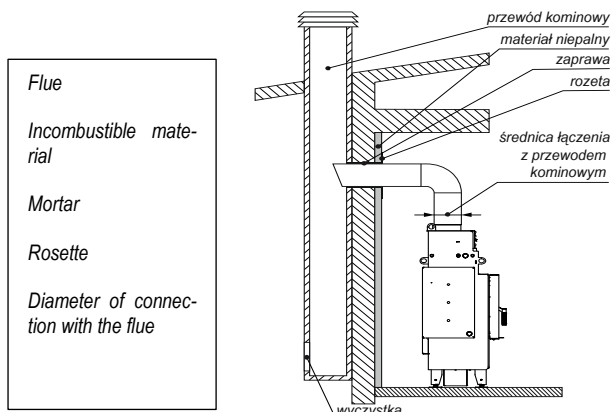
Picture 11. Connection of fireplace inserts to a flue.
