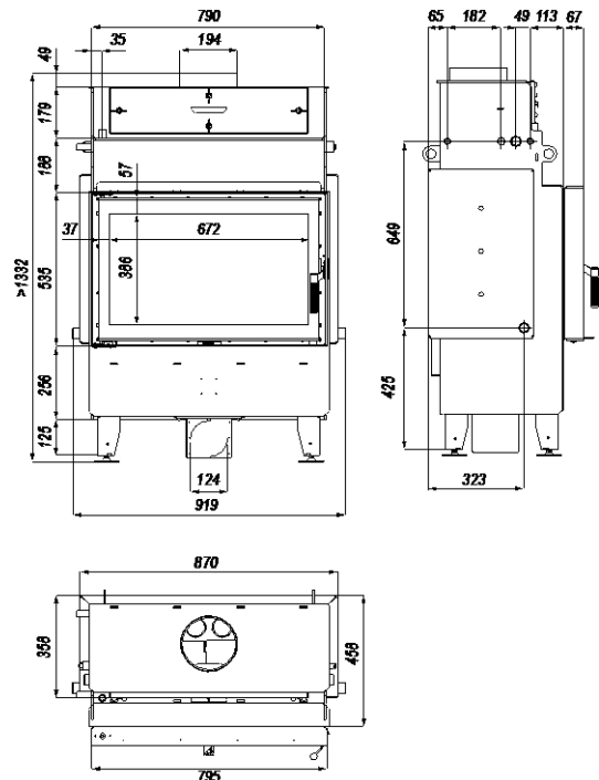
Picture 3. Projections with dimensions of DEFRO HOME NAVI ME fireplace insert.
