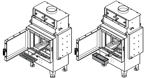
Picture 16. Removal of grate and ash-pan.
