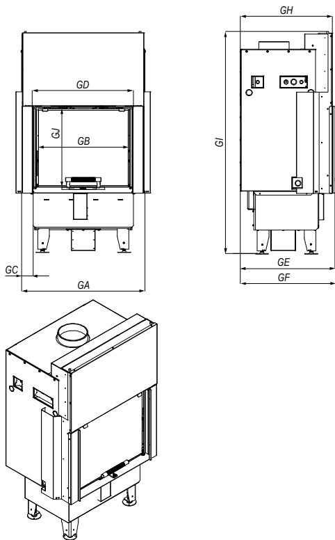
Picture 5 Projections with dimensions of DEFRO HOME NAVI G fire-place insert in version with covers.
