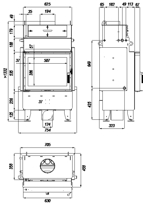
Picture 2. Projections with dimensions of DEFRO HOME NAVI SM fireplace insert.
