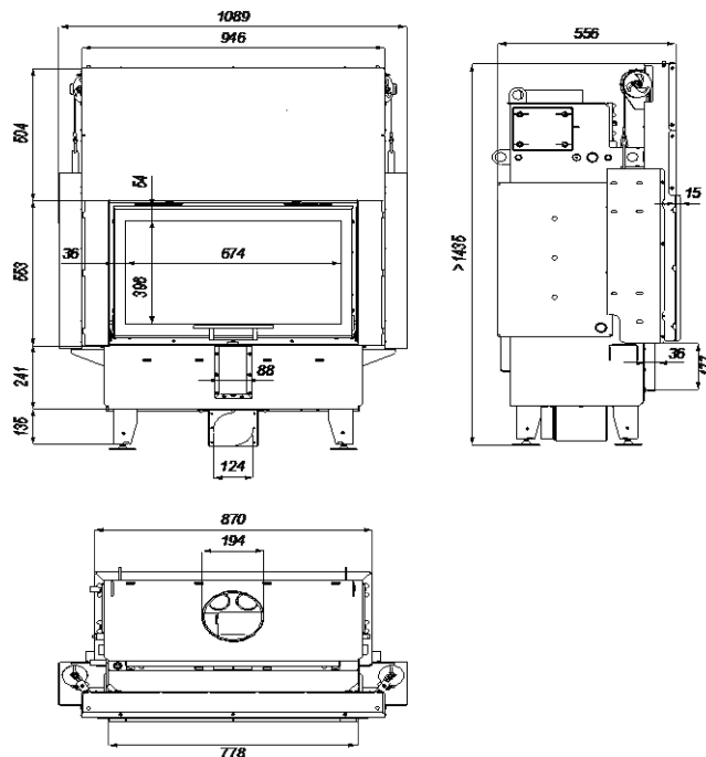
Picture 6 Projections with dimensions of DEFRO HOME NAVI SM G fire-place insert.
