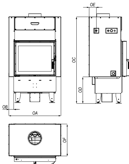
Picture 4.4 Projections with dimensions of DEFRO HOME NAVI fire-place insert in version with covers.
