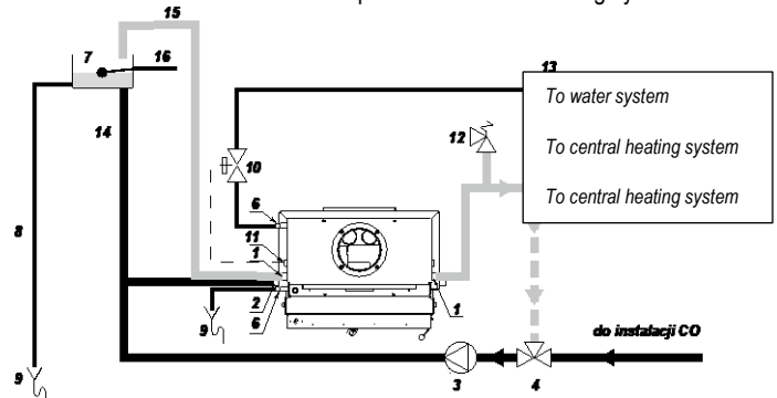
Picture 12 Diagram of exemplary connection of water system of the DEFRO HOME NAVI fireplace with the heating system in the open system.
