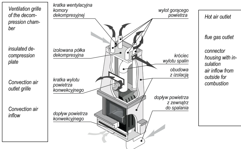
Picture 9 Hot air distribution system.
