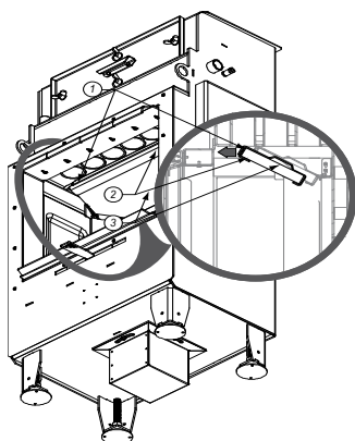
Picture 19. Window panel dismantling from doors.
