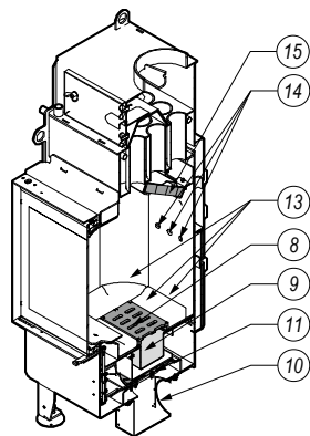
Picture 1. Design of the DEFRO HOME NAVI fireplace insert.
