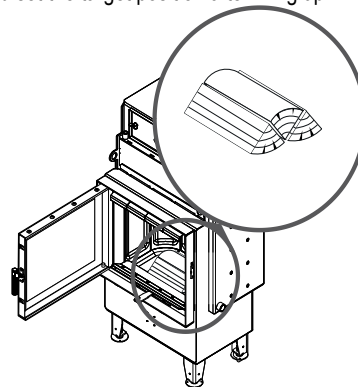
Picture 15. Method of fuel arrangement
