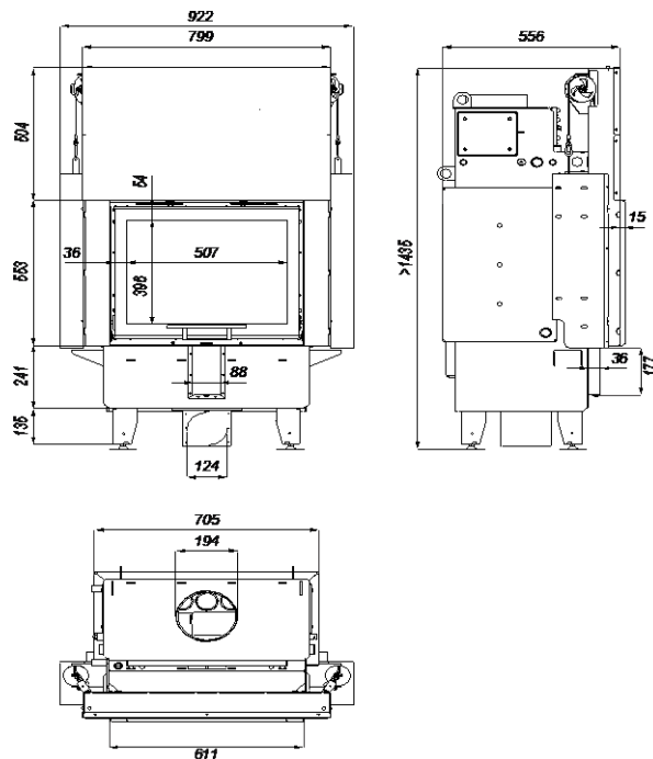
Picture 6 Projections with dimensions of DEFRO HOME NAVI SM G fire-place insert.
