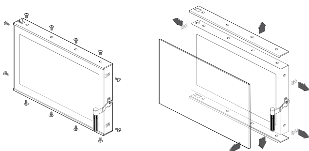
Picture 19. Window panel dismantling from doors.
